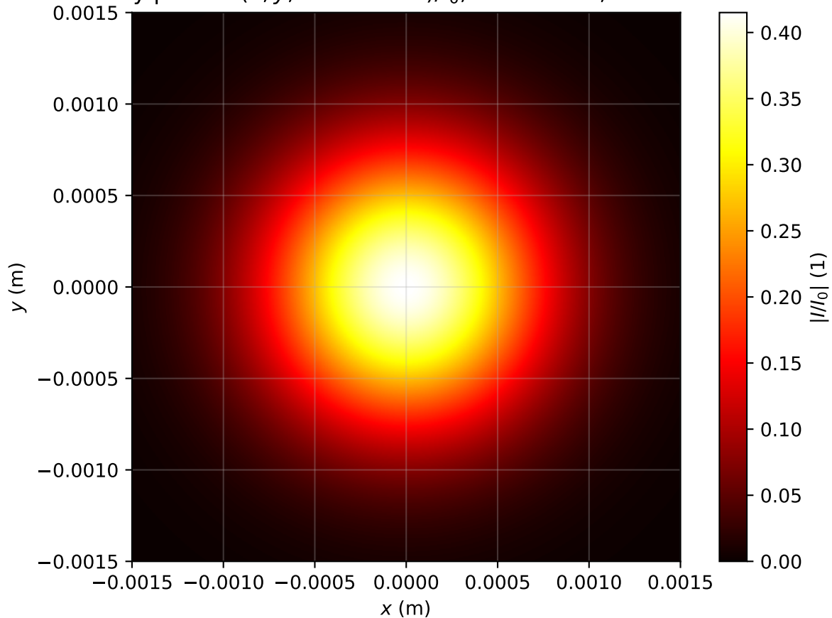
Intensity profile I(x, y, z = 2.548m)/I_0 , P_{in}=0.1P_{cr} , artificial time
